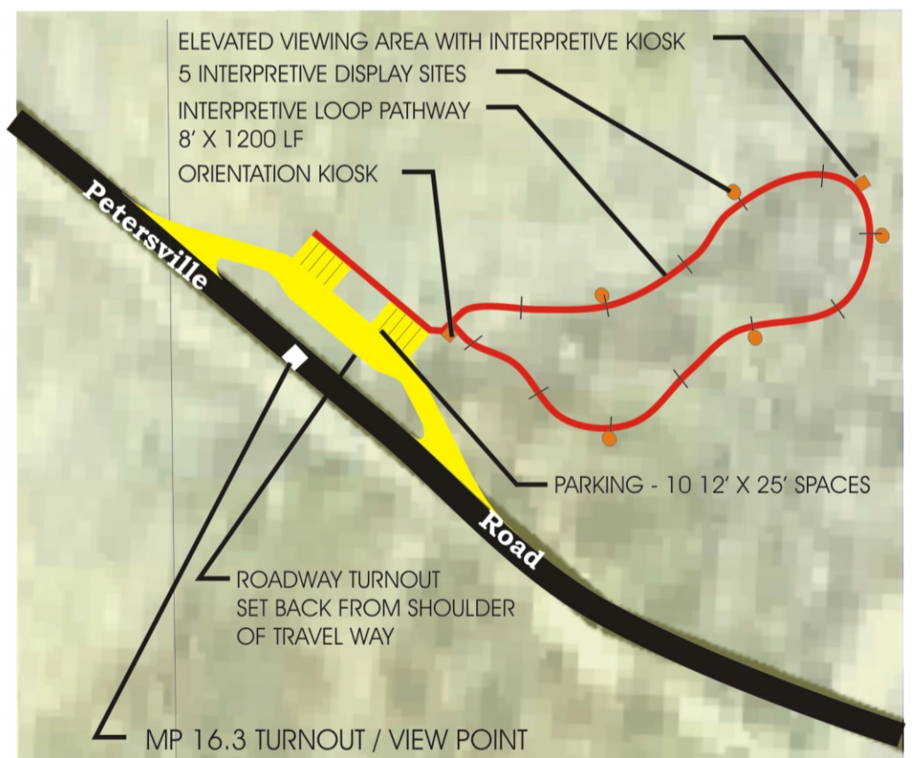
SITE PLAN CONCEPT
