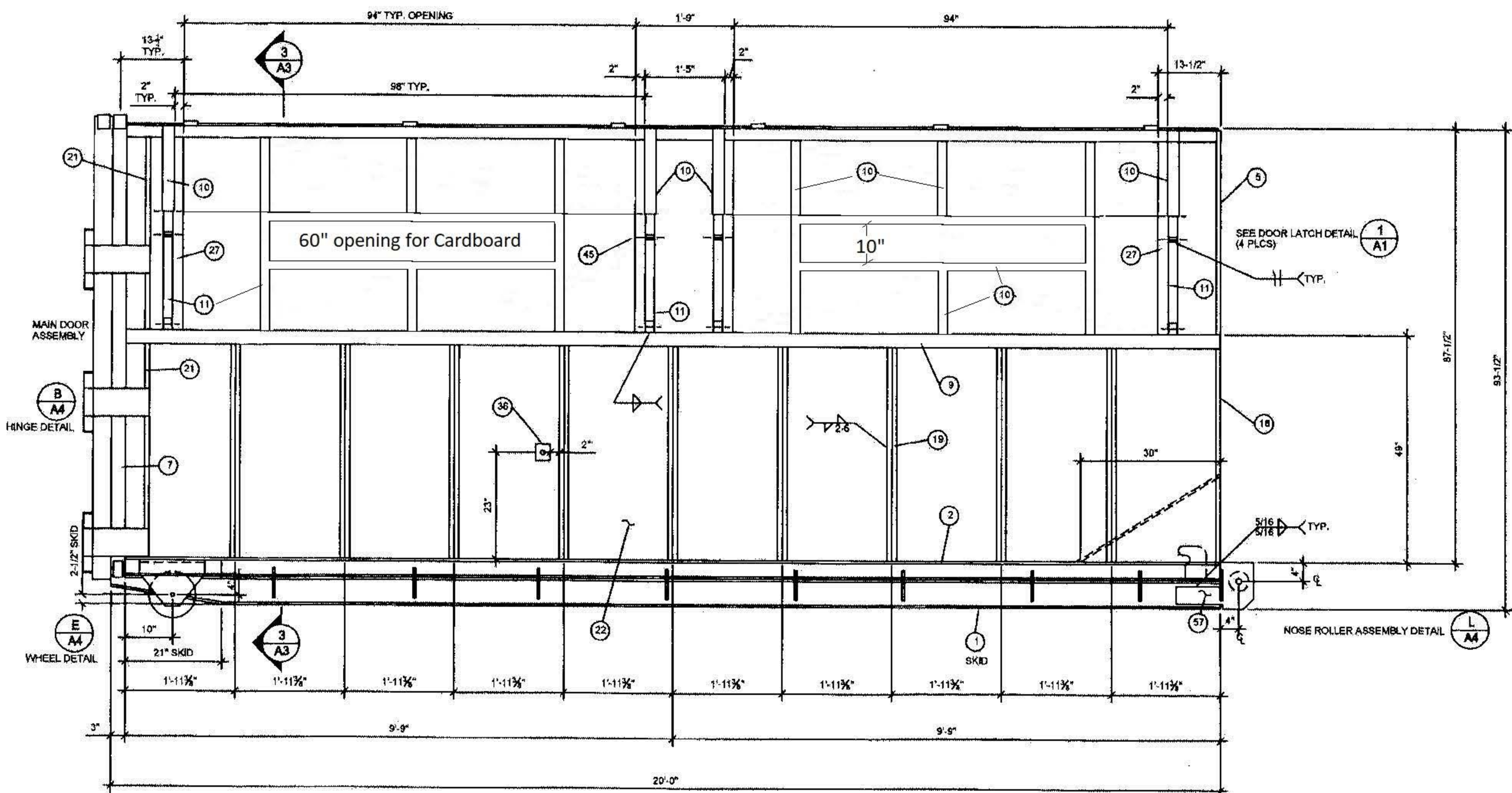
3 RIGHT SIDE VIEW A1 3/4" x 1'-0"
